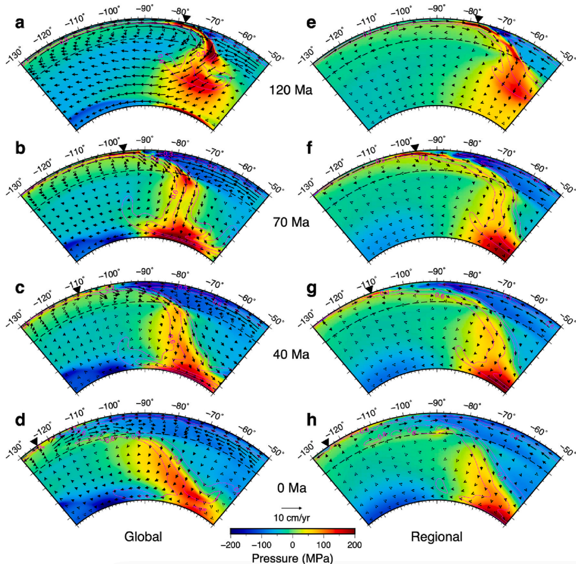
Fig. 7. The evolution of Farallon slab, dynamic pressure, and velocity field in the models beneath North America along 38^{\circ}\text{N} . (a-d) Global model evolution with time snapshots at 120 Ma, 70 Ma, 40 Ma and 0 Ma, respectively. (e-h) The same as (a-d) but for the regional model.
